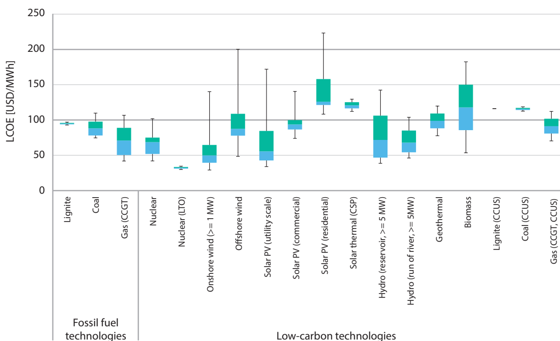
Figure ES1: LCOE by technology
