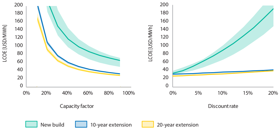
Figure 8.3: Sensitivity of LCOE of new build and LTO of NPPs to capacity factor (left) and discount rate (right)
