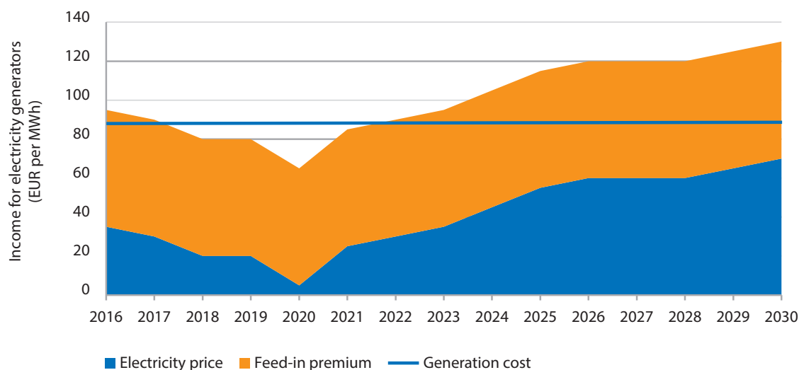
Figure 7.5: Feed-in premium
